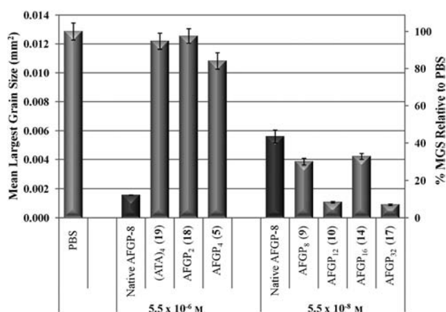
Figure 2. Ice recrystallization inhibition (IRI) activity of isolated AFGP-8, unglycosylated polypeptide (ATA) 4 ( 19 ), AFGP 2 ( 18 ), AFGP 4 ( 5 ), AFGP 8 ( 9 ), AFGP 12 ( 10 ), AFGP 16 ( 14 ), AFGP 32 ( 17 ) at the concentrations given in the figure. The %MGS (mean grain size) of ice crystals relative to the phosphate buffered saline (PBS) positive control is shown for all compounds.
