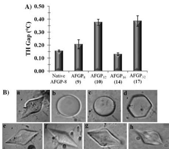
Figure 1. A) Thermal hysteresis (TH) activity of homogeneous synthetic AFGPs and isolated AFGP-8 at 10 mg mL -1 . B) Ice crystal morphology in the presence of: a) native AFGP-8; b) AFGP 2 ( 18 ); c) unglycosylated polypeptide (ATA) 4 ( 19 ; 5 mg mL -1 ); d) AFGP 4 ( 5 ); e) AFGP 8 ( 9 ); f) AFGP 12 ( 10 ); g) AFGP 16 ( 14 ); h) AFGP 32 ( 17 ) at 10 mg mL -1 .
